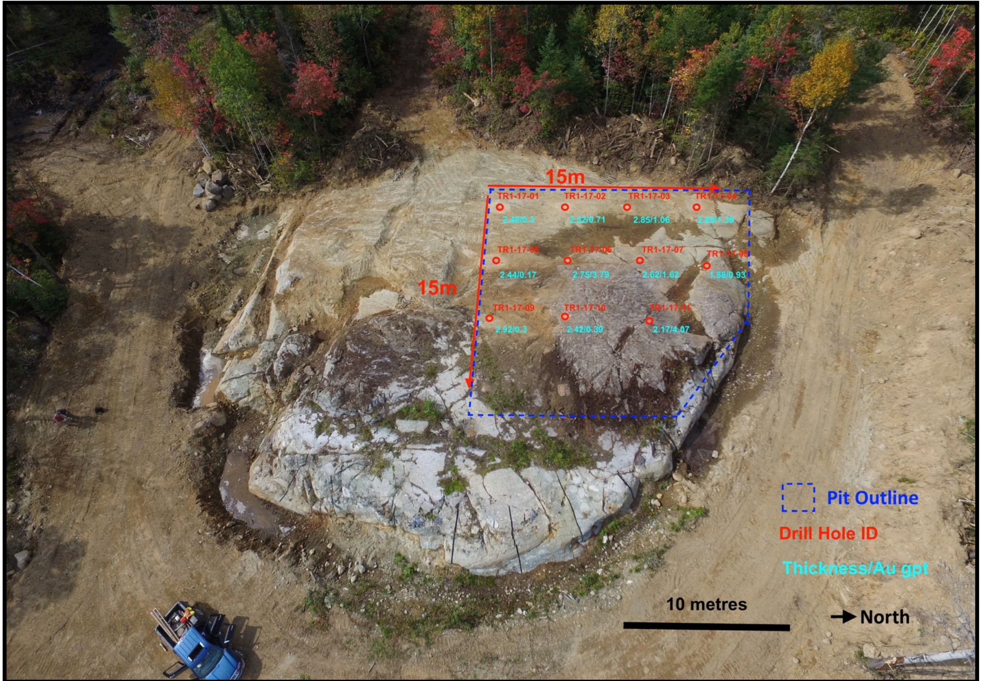
Figure 1 – Trench 1 Bulk Sample Area (Pardo Project) - Jan 3, 2018
